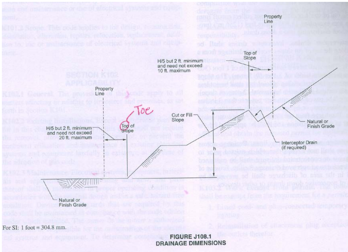
Figure J108.1 DRAINAGE DIMENSIONS (Revise figure as indicated below)
